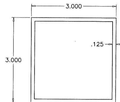
2 X 3 STD. MULLION 6063-T6
