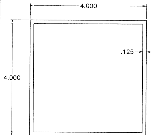
2 X 4 STD. MULLION 6063-T6
