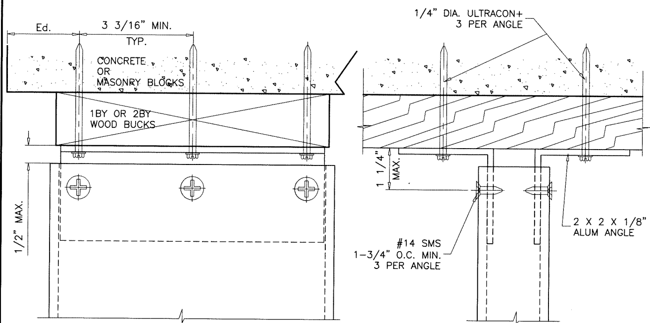
ANCHORS TYPE 'H'
