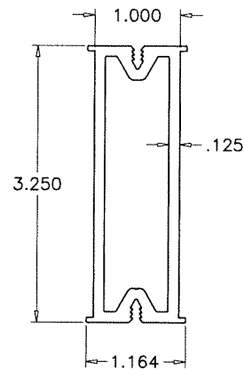
1 X 3 STD. MULLION 6063-T6
