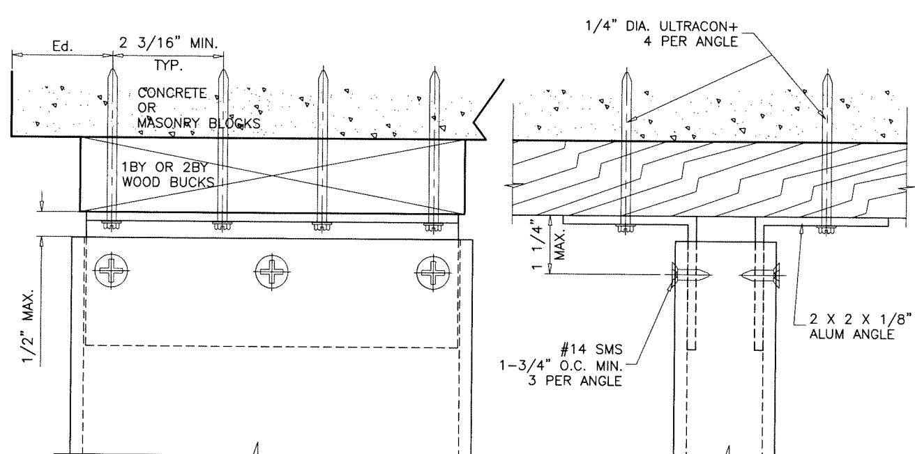
ANCHORS TYPE 'i'
